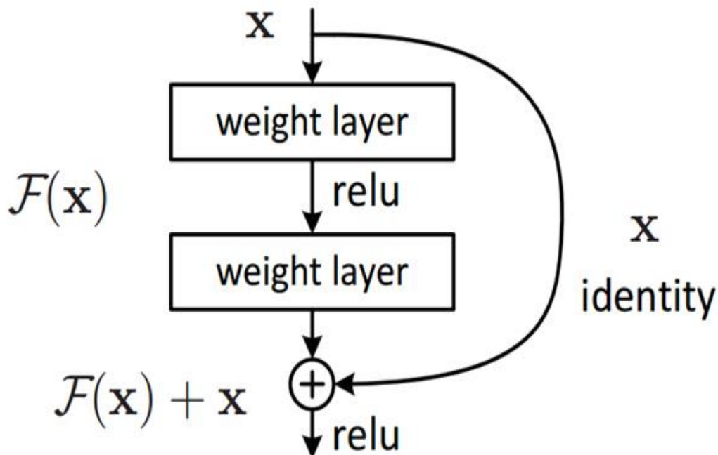
Fig 6: ResNet50 ConvNet
