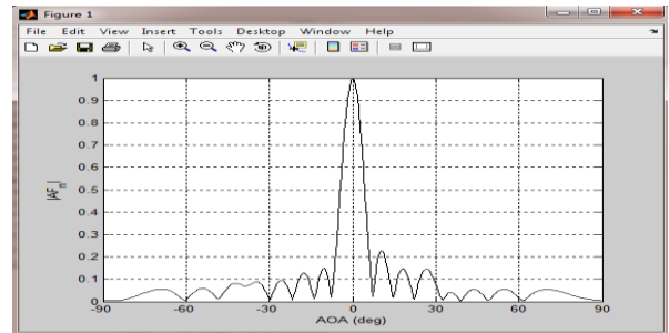
Fig. 6: Normalized Array Factor Plot For Case 2.
