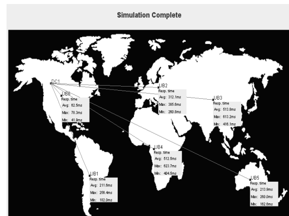
Fig.6 Identifying the popular Data
