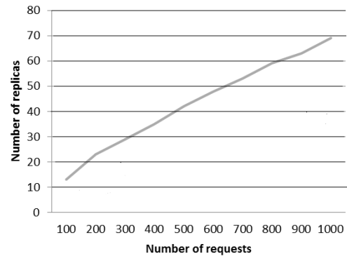
Fig.5 Increasing Number of Requests corresponding Increase Replicas
