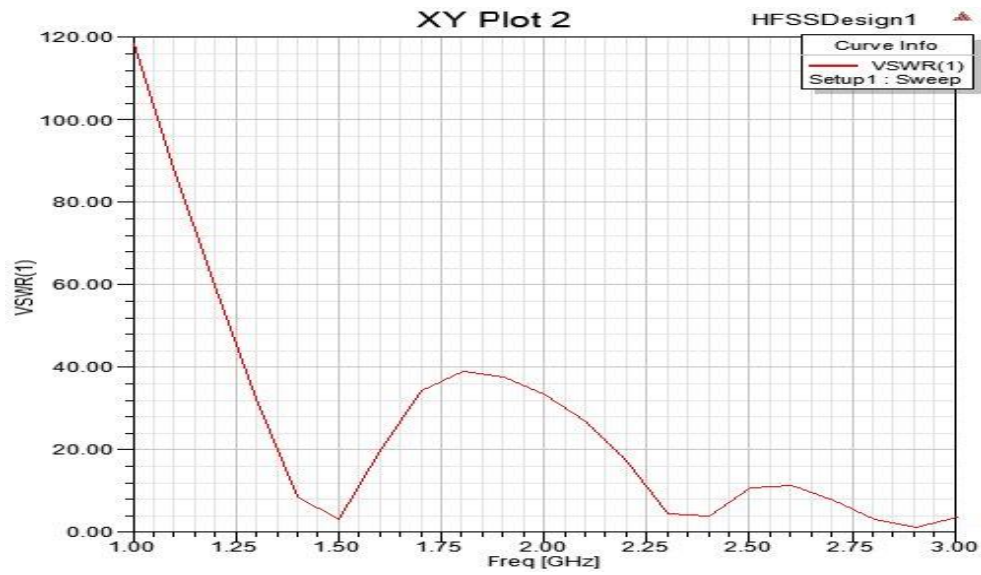
Figure 3: VSWR plot for 1.5GHz.
