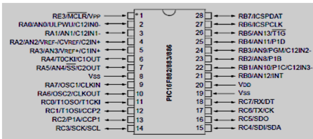
Figure 5: Pin Diagram of PIC16F883 Microcontroller.
