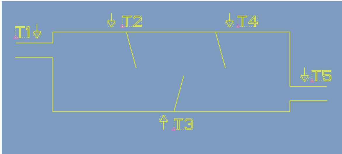
Fig.16: shows muffler with three plates at 15° inclination. T1, T5 are inlet and outlet temperature and T2, T3, T4 are the temperature measured at plates
