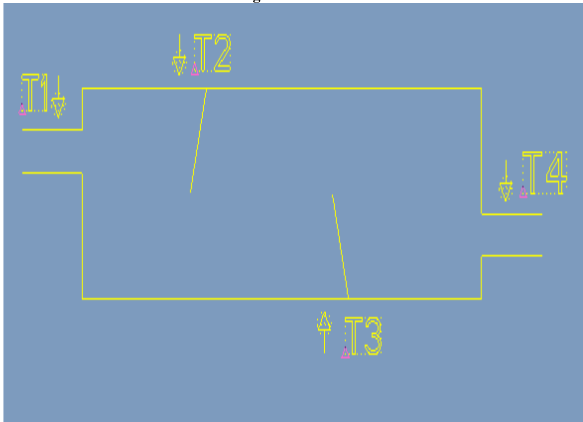
Fig.12: shows muffler with two plates at 15° inclination. T1, T4 are inlet and outlet temperature and T2, T3 are the temperature measured at plates
